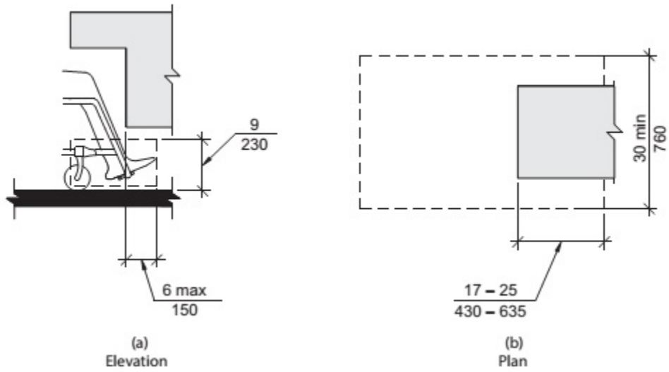
FIGURE 306.2 TOE CLEARANCE
