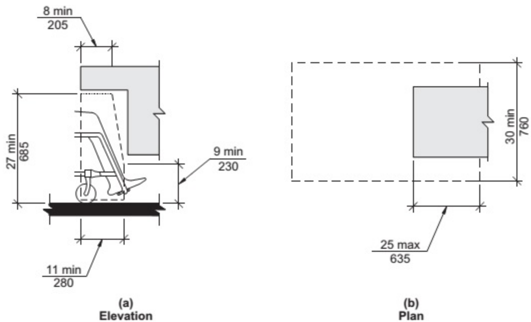
FIGURE 306.3 KNEE CLEARANCE
